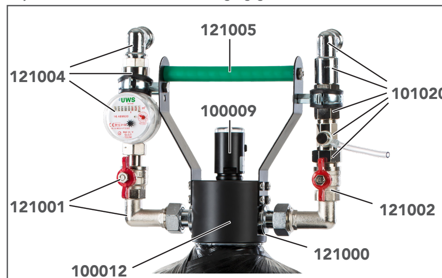
Fig. 6-8: Heaty Small 100 HW reservdelar
