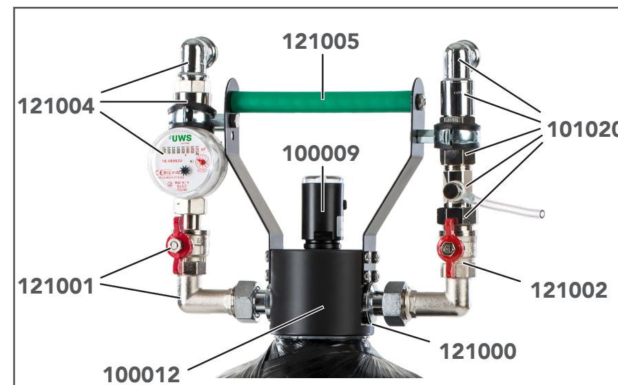
Fig. 6-8: Heaty Small 100 HW reservedele
